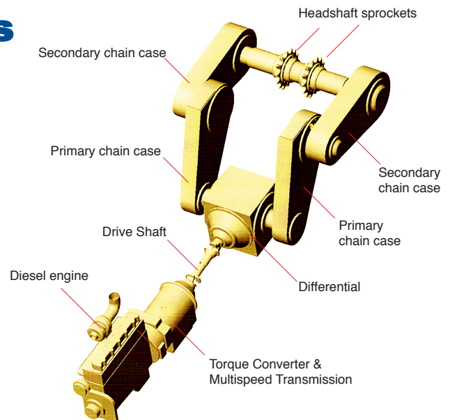
The mechanical chain drive has proven to be much more rugged and trouble free than hydrostatic designs
